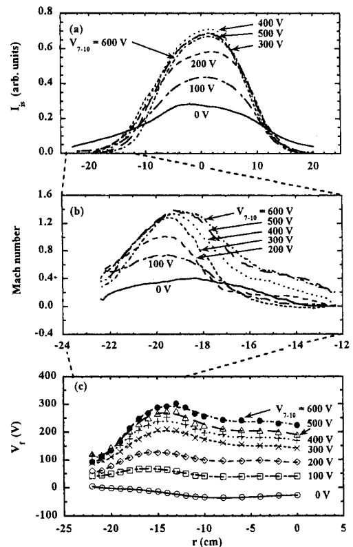
Fig. 2 Radial profile of (a) ion saturation current I_{is} , (b) Mach velocity M and (c) floating potential V_f , changing biased voltage V_{7-10} .
