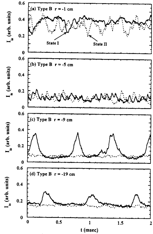
Fig. 4 Time evolution of ion saturation current I_{is} , ( V_3 = 200 V) for the radial location r of (a) -1 cm, (b) -5 cm, (c) -9 cm and (d) -19 cm (Eight individual traces have different shots).
