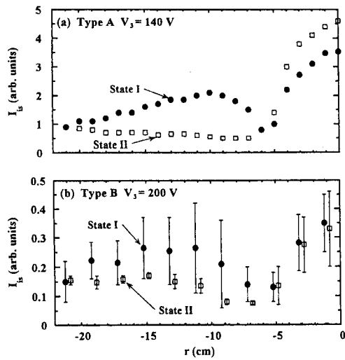
Fig. 5 Radial profile of ion saturation current I_{is} in the (a) Type A and (b) Type B transitions. Here, vertical lines indicate typical fluctuation amplitude of I_{is} .
