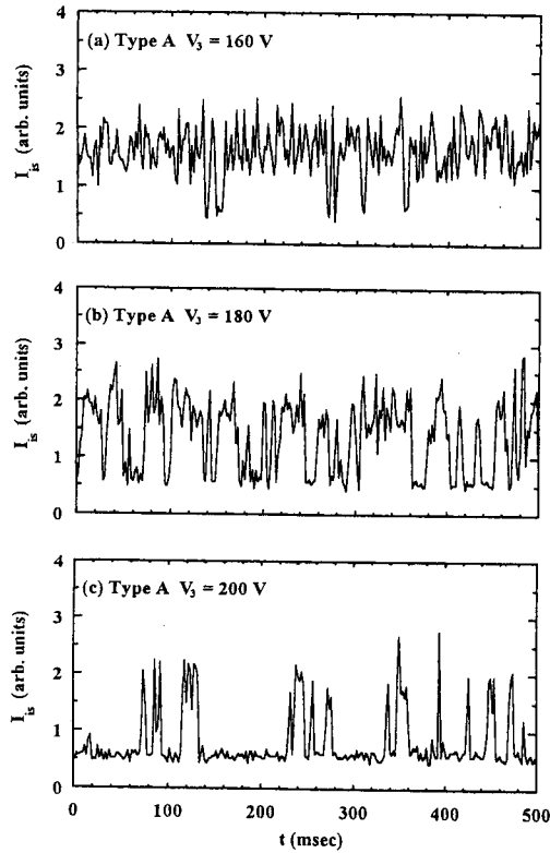
Fig. 3 Time evolution of ion saturation current I_{is} ( r = -13 cm), for the biased voltage V_3 of (a) 160 V, (b) 180 V and (c) 200 V (they were different shots).
